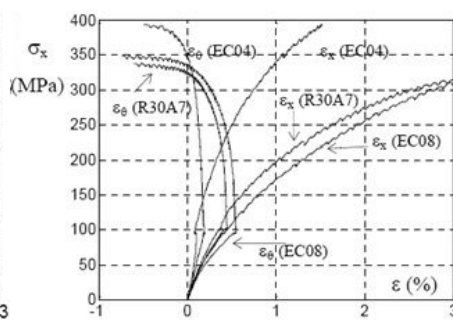
Figure 9. Triaxial tests with p=100 MPa: axial stress versus strain components for E/C values of 0.4, 0.64 and 0.8.
