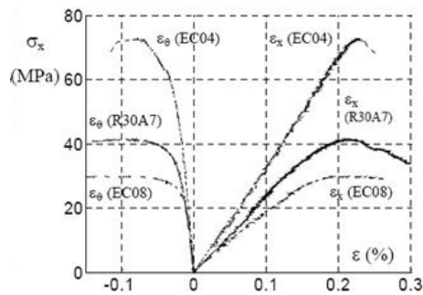
Figure 8. Uniaxial compression tests: axial stress versus strain components for E/C values of 0.4, 0.64 and 0.8.
