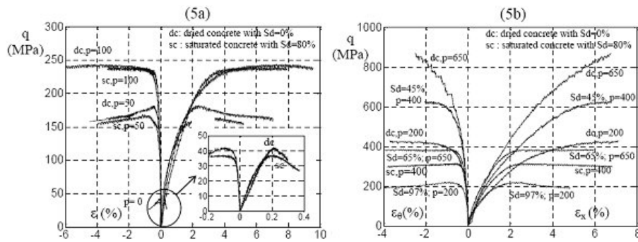
Figure 5. Triaxial tests - dried and partially saturated concrete: principal stress difference versus strain components for a confining pressure from 0 to 100 MPa (5a), and from 200 to 650 MPa (5b).
