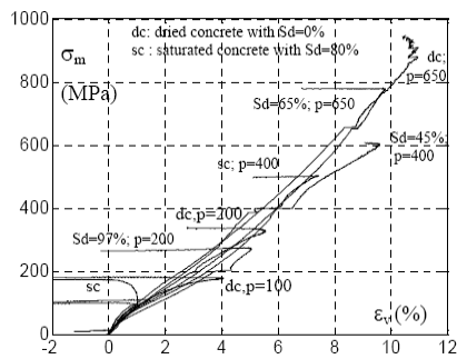
Figure 6. Triaxial tests on the dried and partially saturated concretes R30A7: mean stress versus the volumetric strain.
