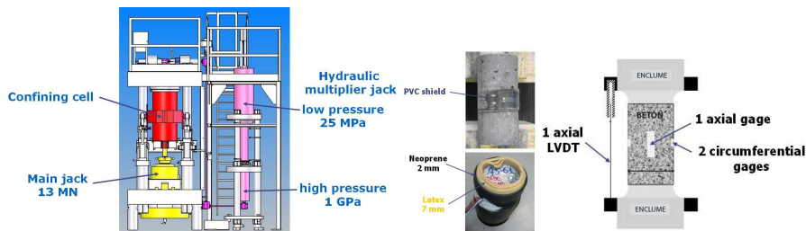
Figure 1. General scheme of the press.
