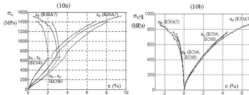
Figure 10. Triaxial tests with p=650 MPa: stress/strain curves (a), principal stress difference/strain curves (b) for E/C values of 0.4, 0.64 and 0.8.
