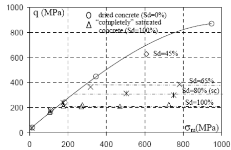
Figure 7. Limit states of the dried and saturated concrete in the stress invariant space ( \sigma_m , q_{max} ).
