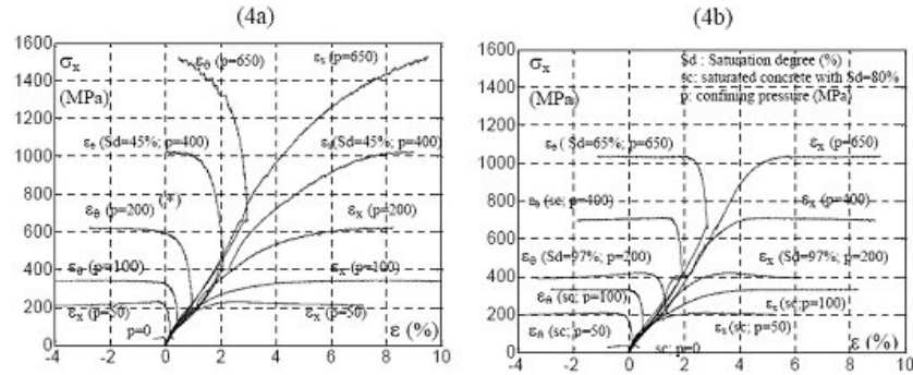
Figure 4. Triaxial tests on the dried concrete R30A7 (4a) and the partially saturated concrete R30A7 (4b) : stress/strain curves S_d : Saturation degree ( S_d=0\% for “completely” dried concrete and S_d=100\% for “completely” saturated concrete); sc : saturated concrete with S_d=80\% ; p : confining pressure in the triaxial test (MPa).
